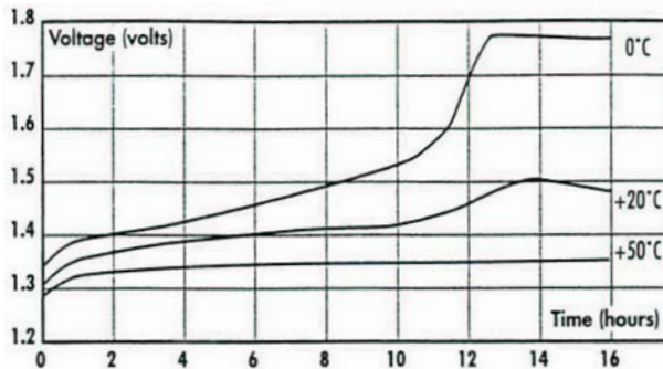
Voltage in normal charge current 0.1 C
