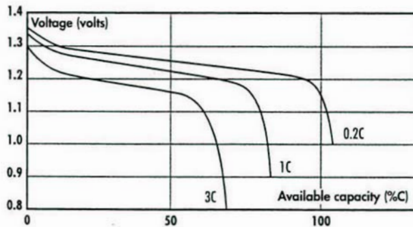
Voltage in discharge at +20 °C after charge 0.1 C x 16 hours at +20 °C
