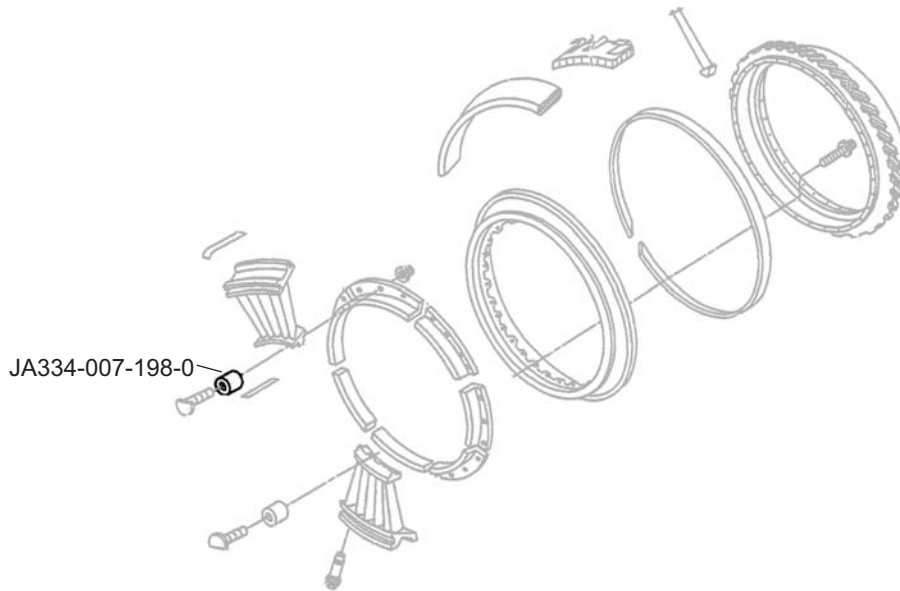
Oversized Bushing
